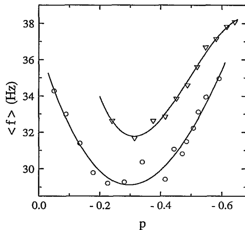
FIG. 3. First moment \langle f \rangle of the NMR line shapes as a function of p , measured in zero field (O) and at B_y = 5 \mu\text{T} ( \nabla ). The curves are just to guide the eyes.
