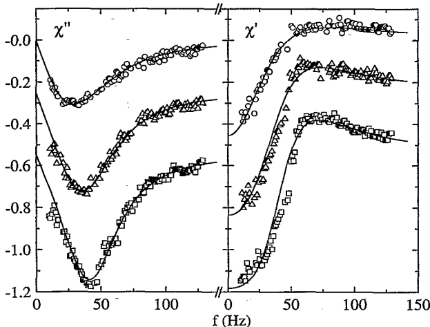
FIG. 1. NMR absorption \chi'' and dispersion \chi' curves (in dimensionless SI units) of the nuclear spin system in silver at T < 0 , measured in zero field at reduced entropies S/\mathcal{R} \ln 2 equal to 0.87 ( \circ ), 0.80 ( \Delta ), and 0.73 ( \square ), which correspond to polarizations p = -0.42 , -0.51 , and -0.59 in the paramagnetic state, respectively. The zeros for the lower curves have been shifted downwards by 0.25 and 0.55 in both frames.
