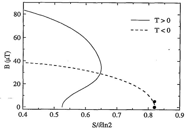
FIG. 4. Phase diagram in the B vs S/\mathcal{R}\ln 2 plane for the nuclear spins in silver metal at negative absolute temperatures. Solid circles represent our experimental data, obtained from Fig. 2, and the dashed curve displays a theoretical phase boundary between the ferromagnetic (at left) and paramagnetic regions. The shape of this curve is based on the mean-field theory [11] with the assumption of a linear relationship between S and T . The antiferromagnetic phase transition curve at T > 0 [2], marked by the solid line, is included for comparison.
