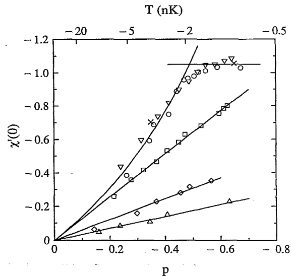
FIG. 2. Static susceptibility \chi'(0) vs polarization p of silver nuclear spins at T < 0 , measured in a magnetic field B_y of 0 ( \circ ), 5 ( \nabla ), 20 ( \square ), 50 ( \diamond ), and 100 \mu\text{T} ( \Delta ), and at B_z = 5 \mu\text{T} ( \times ). The fitted curves are discussed in the text. The scale on top gives estimated temperatures based on the formula [9] 1/|p| - 1 = 0.55|T| (in nK), which applies only at B = 0 ; values to the right of -2 nK must be considered tentative.
